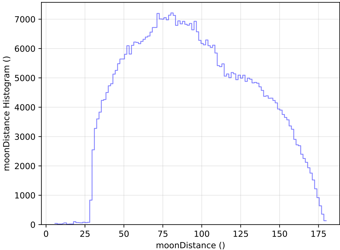
too_elab_r8_d3_gz_v3.4_10yrs WFD i band: moonDistance Histogram
