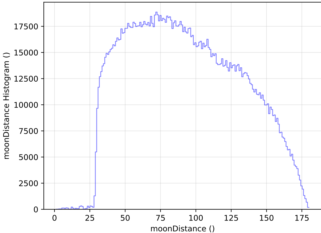
too_elab_r8_d3_gz_v3.4_10yrs WFD all bands: moonDistance Histogram
