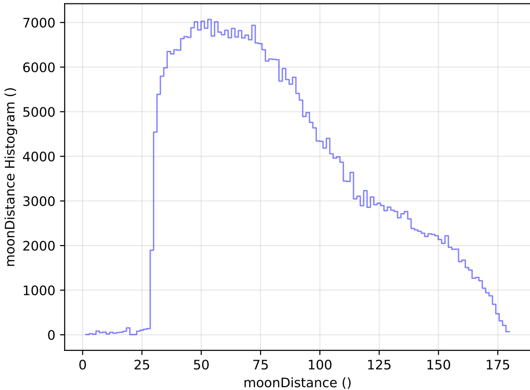
too_elab_r8_d3_gz_v3.4_10yrs All sky z band: moonDistance Histogram
