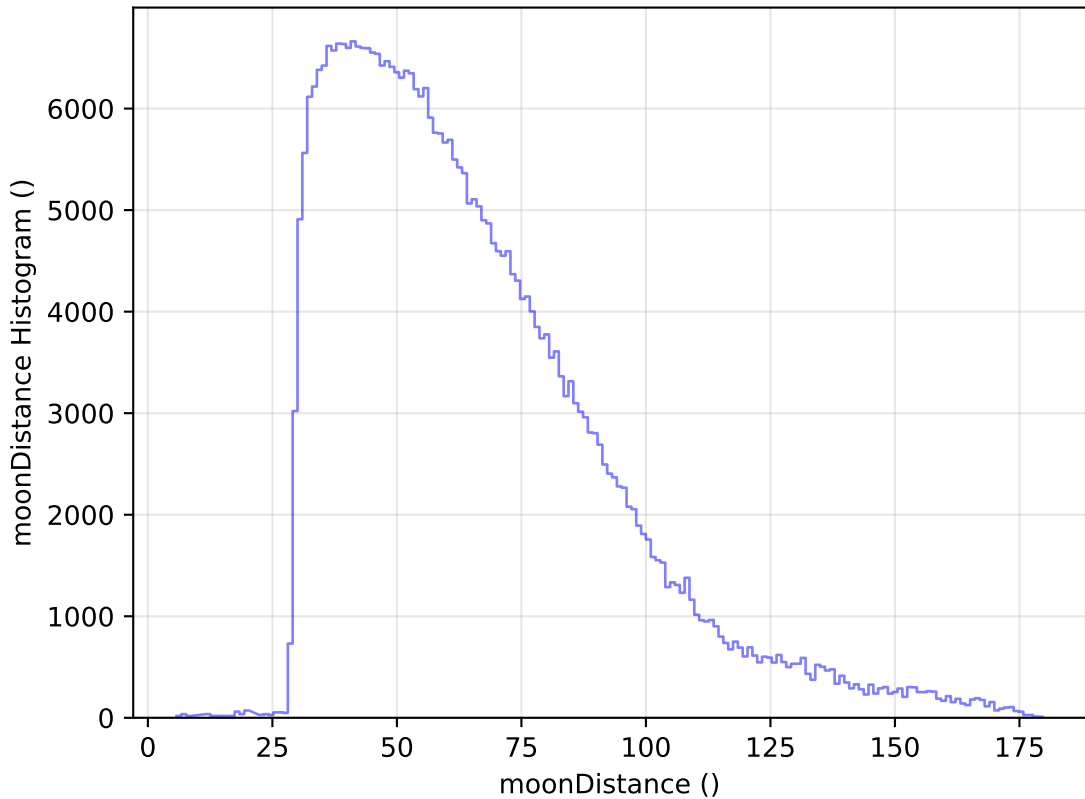
too_elab_r8_d3_gz_v3.4_10yrs All sky y band: moonDistance Histogram
