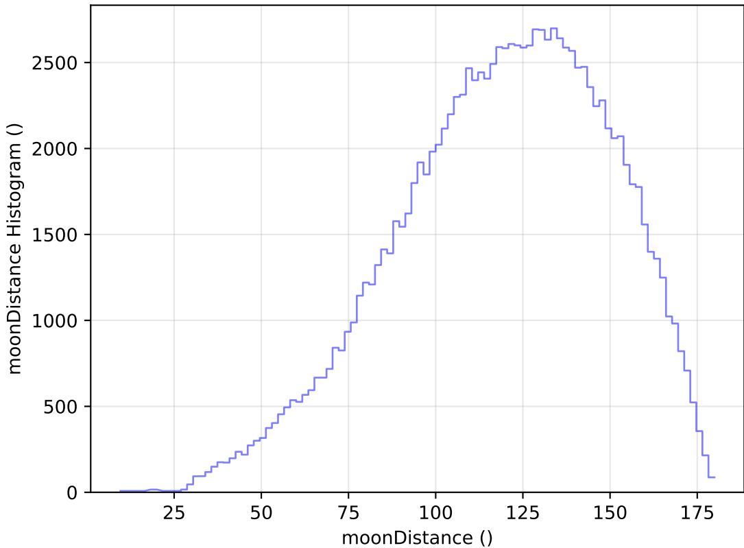
too_elab_r8_d3_gz_v3.4_10yrs All sky u band: moonDistance Histogram
