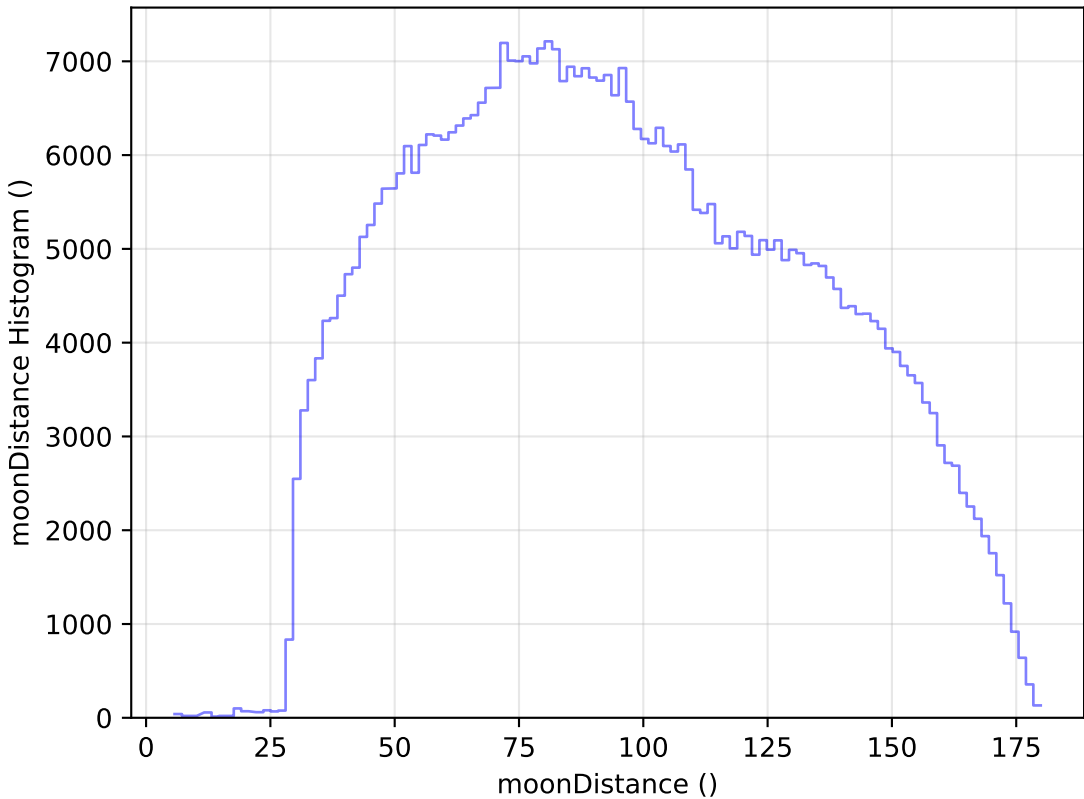
too_elab_r8_d3_gz_v3.4_10yrs All sky i band: moonDistance Histogram
