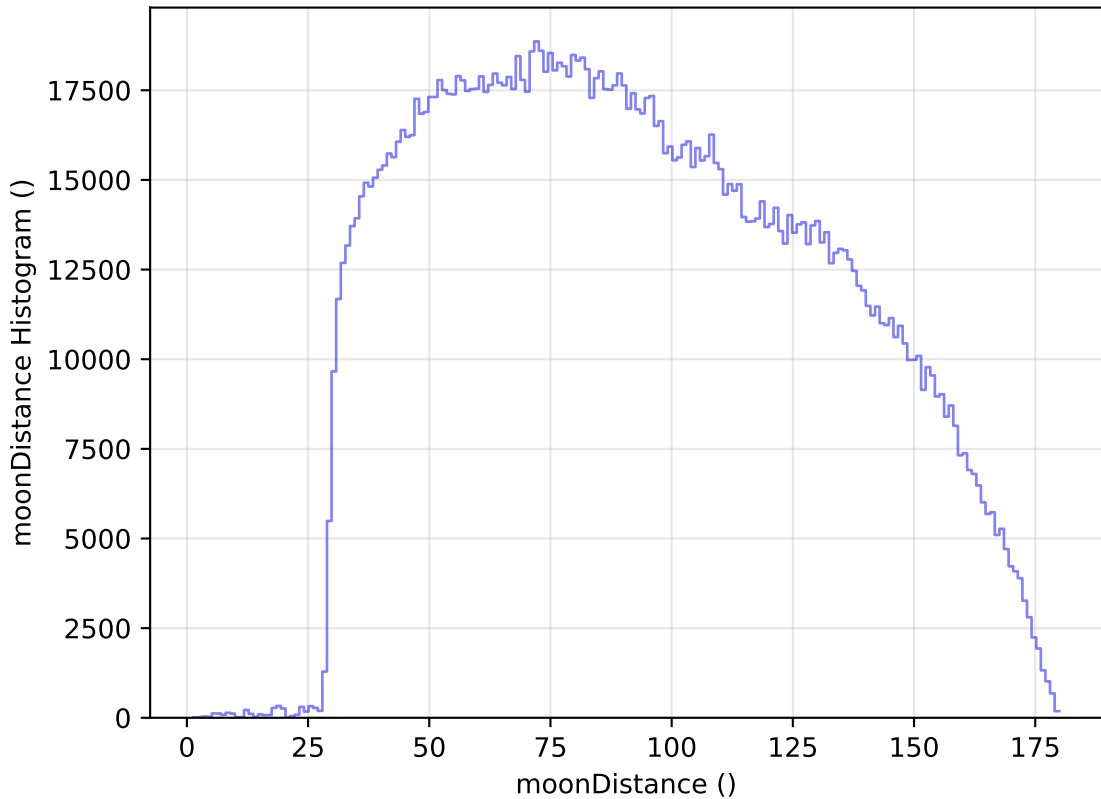
too_elab_r8_d3_gz_v3.4_10yrs All sky all bands: moonDistance Histogram
