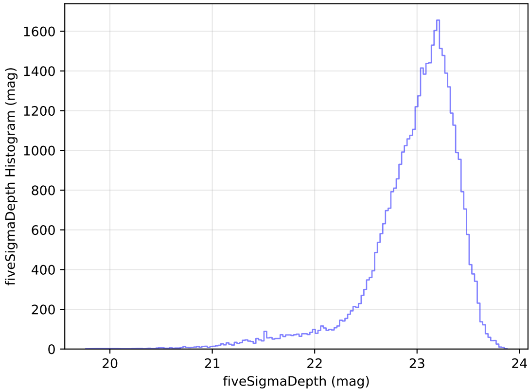
too_elab_r8_d3_gz_v3.4_10yrs Yr 1 z band: fiveSigmaDepth Histogram
