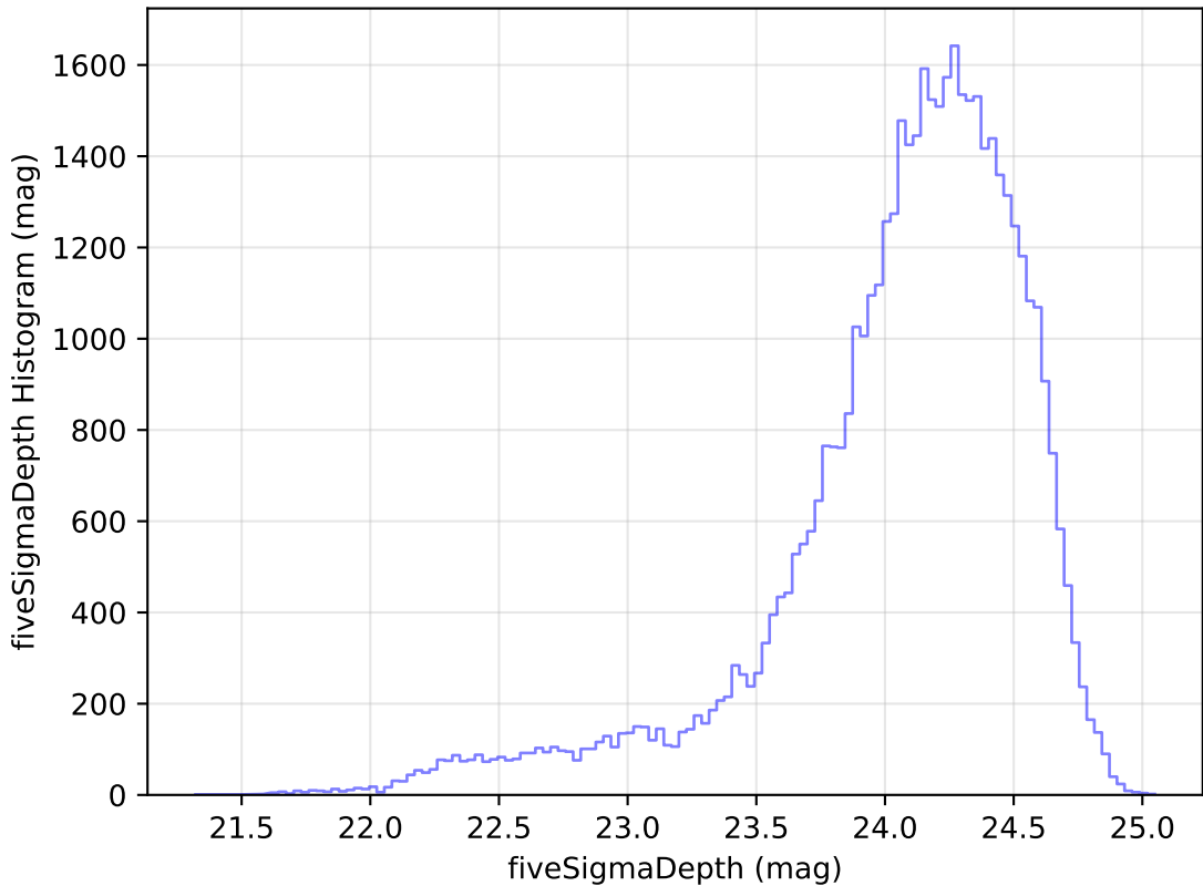
too_elab_r8_d3_gz_v3.4_10yrs Yr 1 r band: fiveSigmaDepth Histogram
