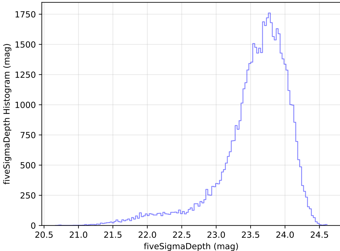
too_elab_r8_d3_gz_v3.4_10yrs Yr 1 i band: fiveSigmaDepth Histogram
