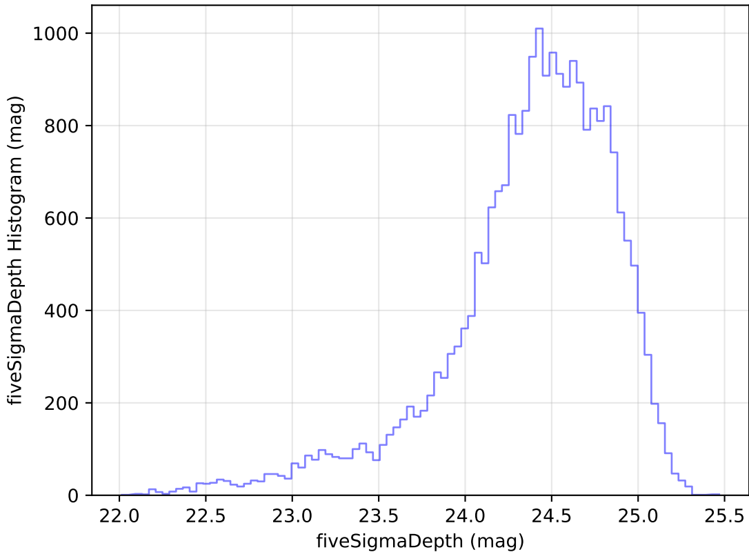
too_elab_r8_d3_gz_v3.4_10yrs Yr 1 g band: fiveSigmaDepth Histogram
