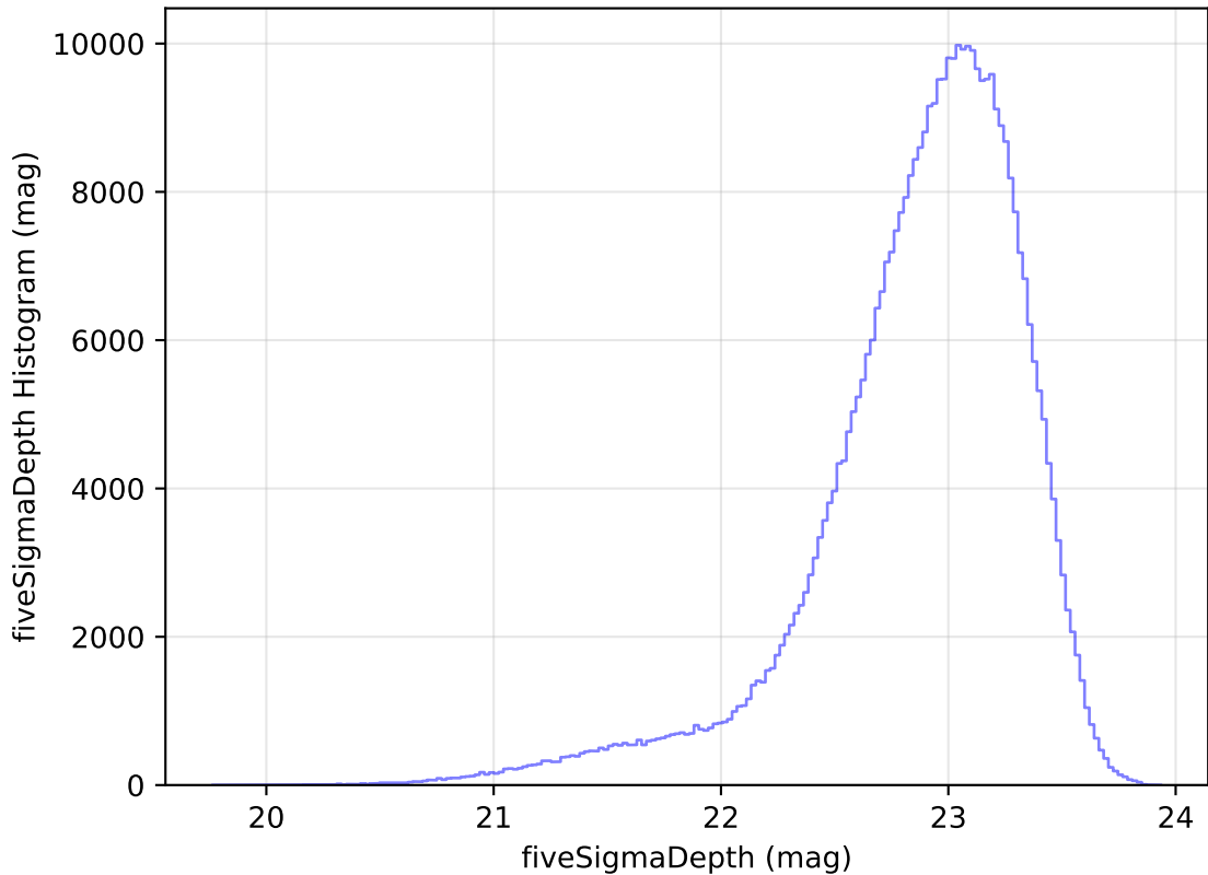
too_elab_r8_d3_gz_v3.4_10yrs WFD z band: fiveSigmaDepth Histogram
