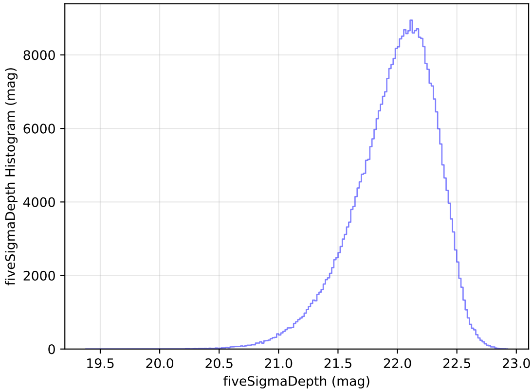
too_elab_r8_d3_gz_v3.4_10yrs WFD y band: fiveSigmaDepth Histogram
