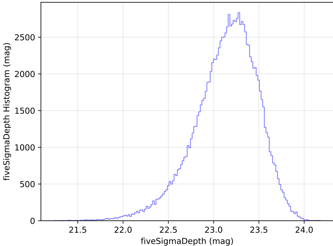
too_elab_r8_d3_gz_v3.4_10yrs WFD u band: fiveSigmaDepth Histogram
