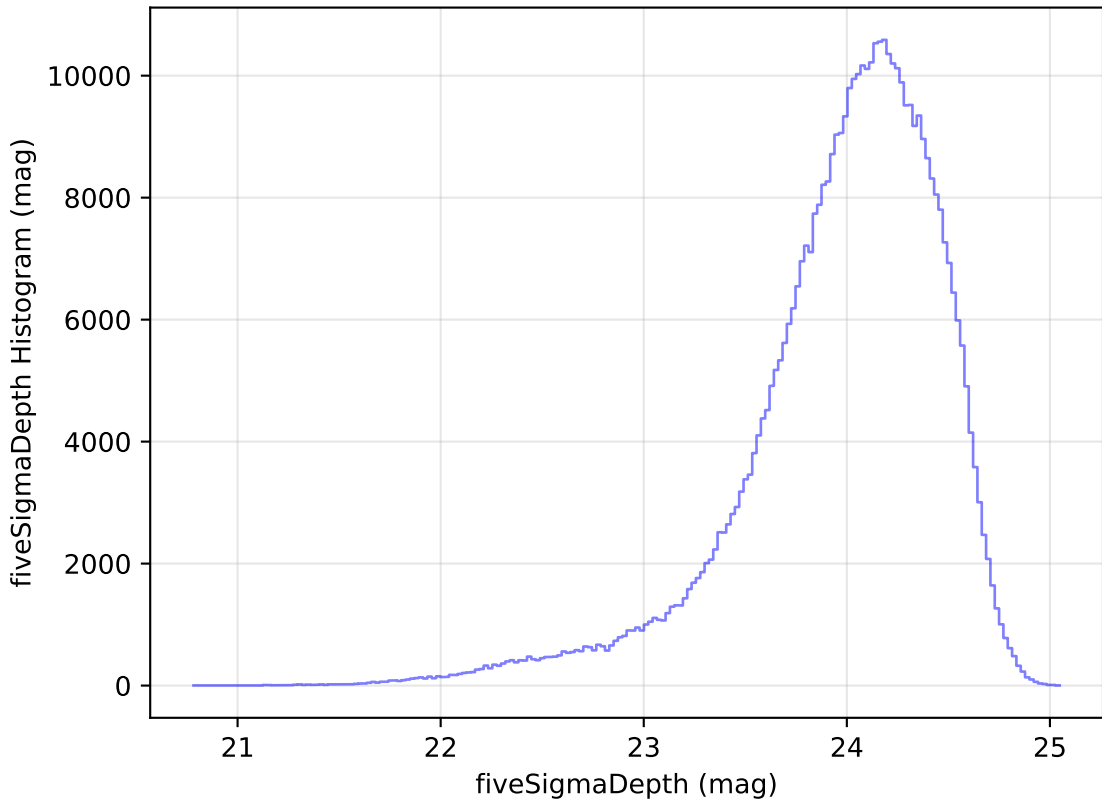
too_elab_r8_d3_gz_v3.4_10yrs WFD r band: fiveSigmaDepth Histogram
