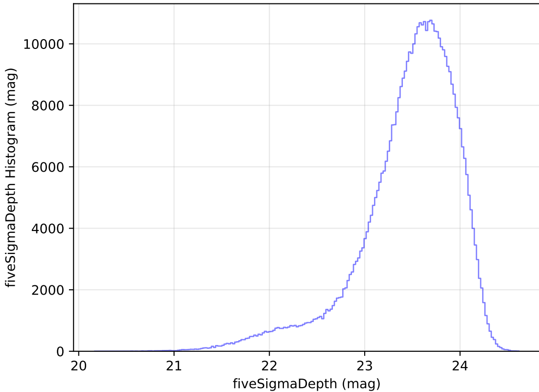
too_elab_r8_d3_gz_v3.4_10yrs WFD i band: fiveSigmaDepth Histogram
