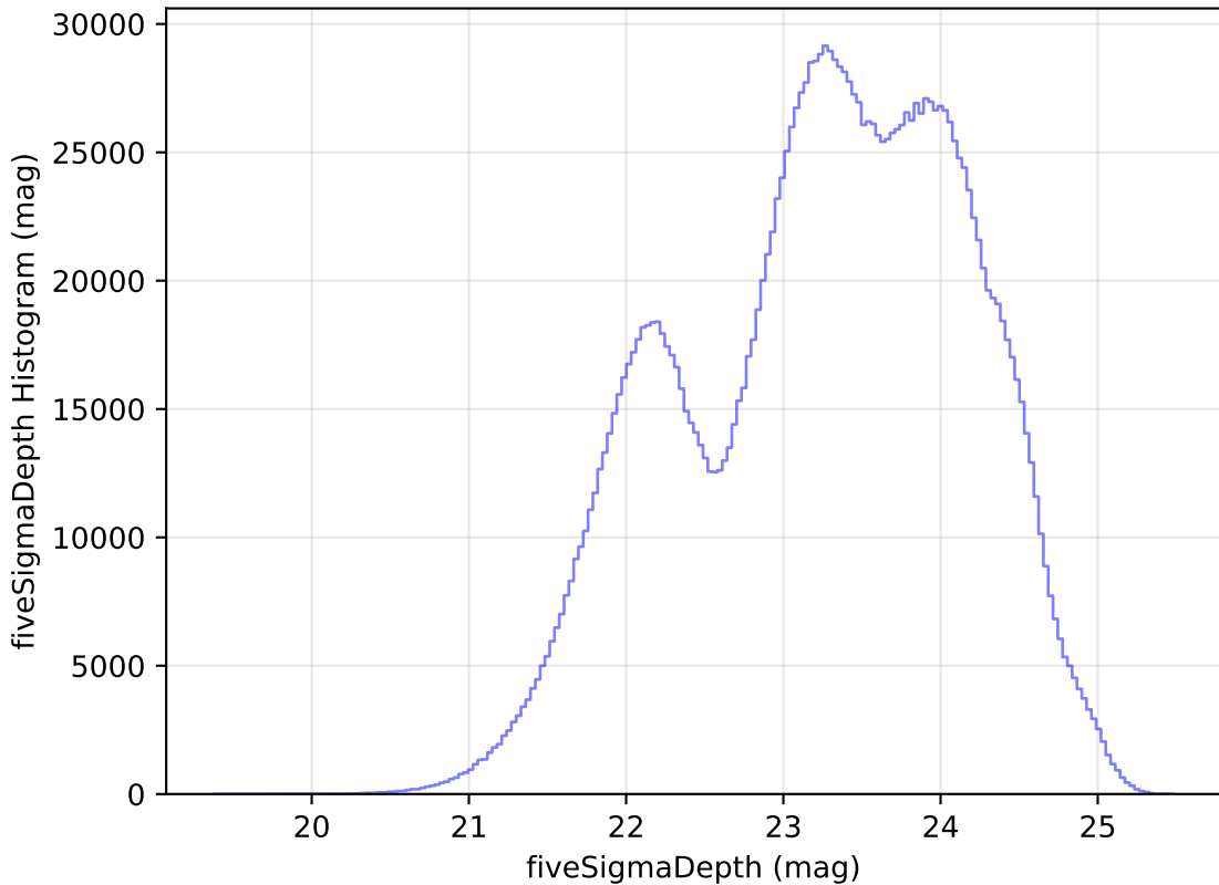
too_elab_r8_d3_gz_v3.4_10yrs WFD all bands: fiveSigmaDepth Histogram
