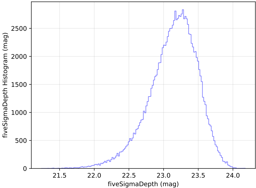
too_elab_r8_d3_gz_v3.4_10yrs All sky u band: fiveSigmaDepth Histogram
