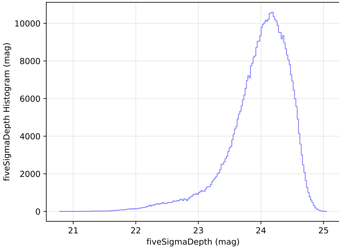
too_elab_r8_d3_gz_v3.4_10yrs All sky r band: fiveSigmaDepth Histogram
