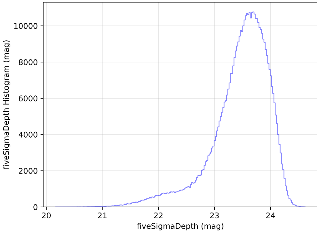
too_elab_r8_d3_gz_v3.4_10yrs All sky i band: fiveSigmaDepth Histogram
