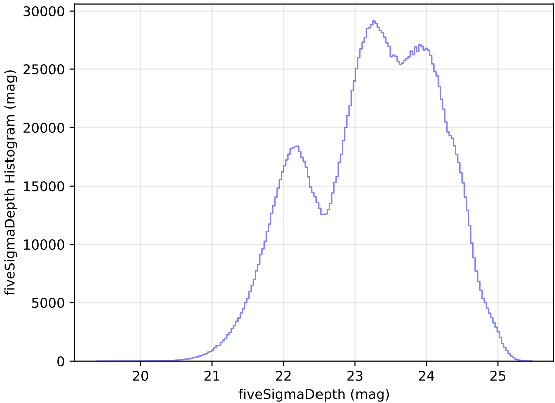
too_elab_r8_d3_gz_v3.4_10yrs All sky all bands: fiveSigmaDepth Histogram
