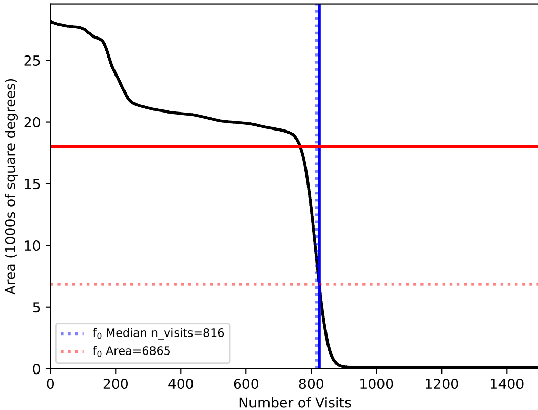
too_elab_r8_d3_gz_v3.4_10yrs All sky: f0
