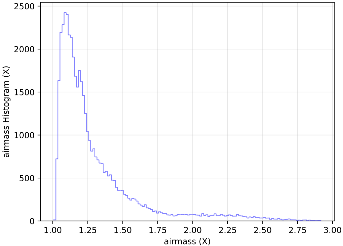
too_elab_r8_d3_gz_v3.4_10yrs Yr 1 z band: airmass Histogram
