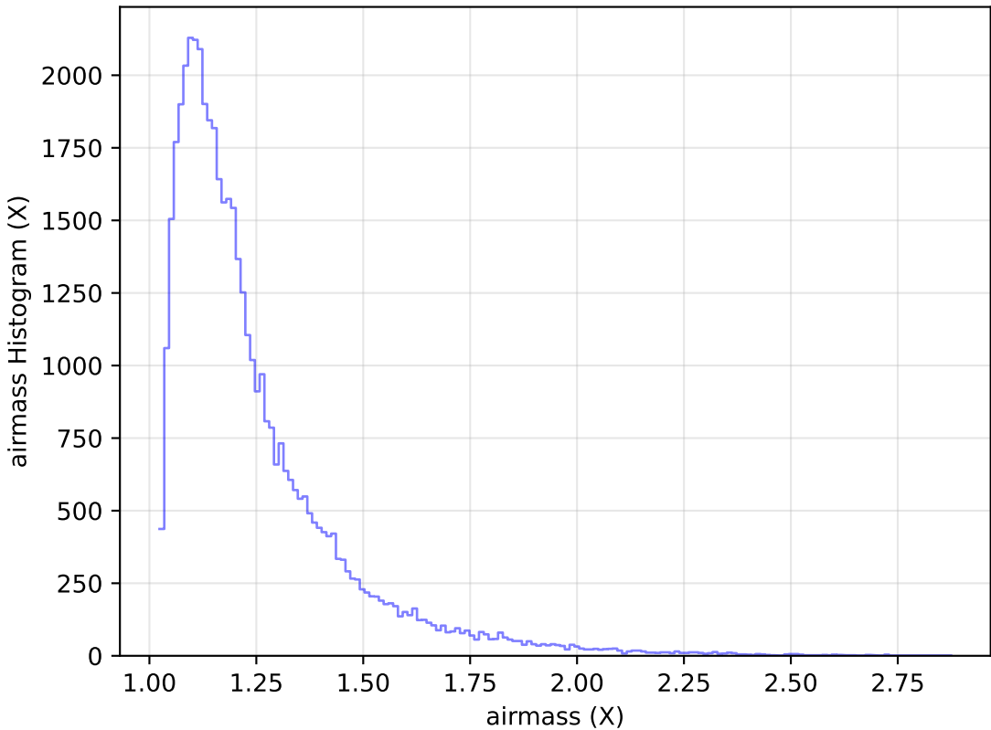
too_elab_r8_d3_gz_v3.4_10yrs Yr 1 y band: airmass Histogram
