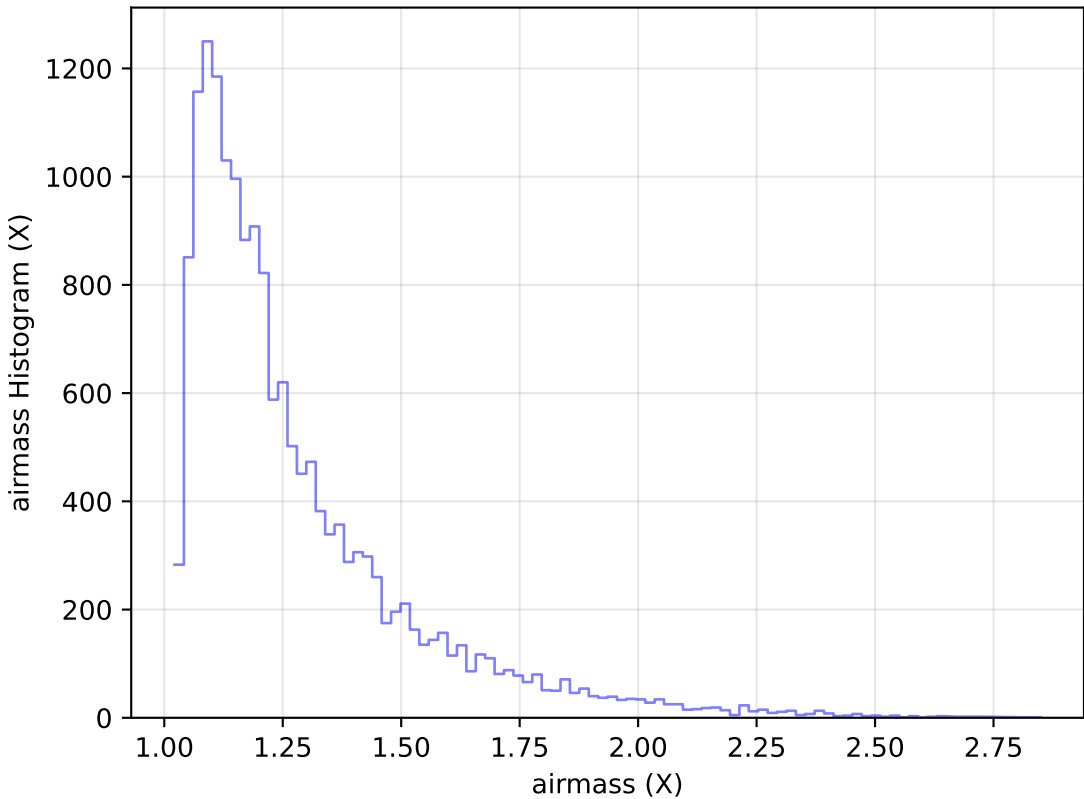
too_elab_r8_d3_gz_v3.4_10yrs Yr 1 u band: airmass Histogram
