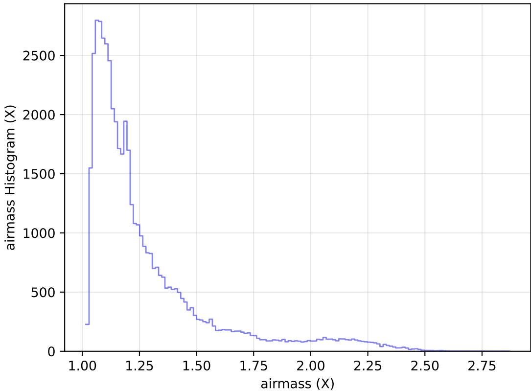
too_elab_r8_d3_gz_v3.4_10yrs Yr 1 r band: airmass Histogram
