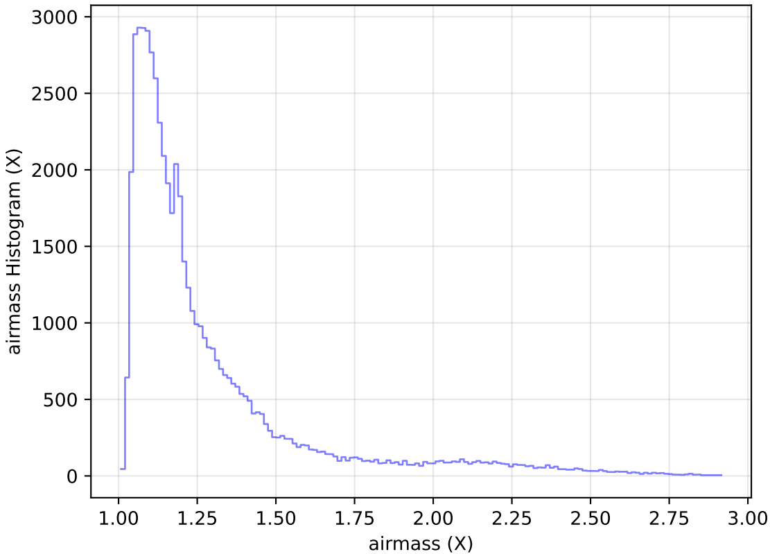
too_elab_r8_d3_gz_v3.4_10yrs Yr 1 i band: airmass Histogram
