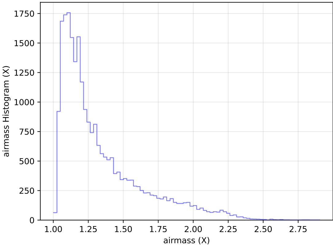
too_elab_r8_d3_gz_v3.4_10yrs Yr 1 g band: airmass Histogram
