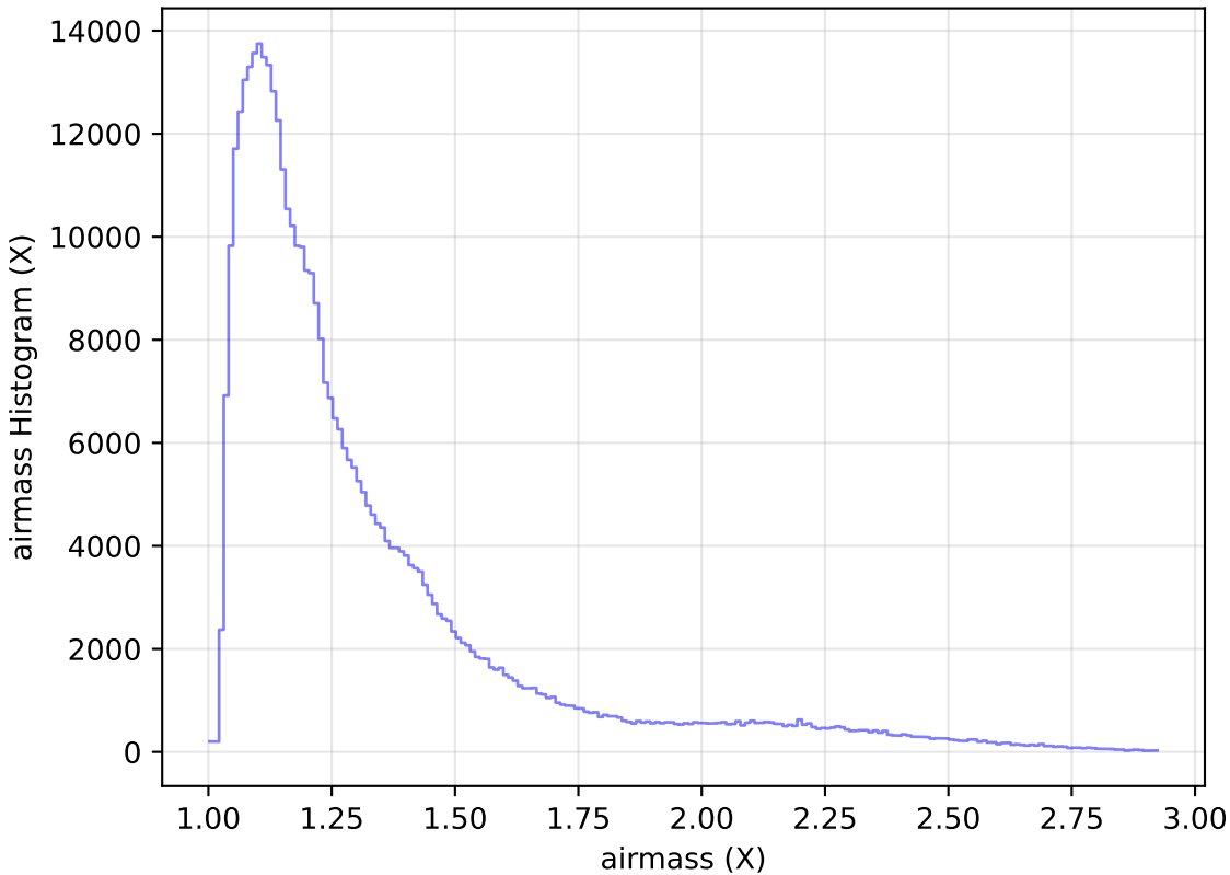
too_elab_r8_d3_gz_v3.4_10yrs WFD z band: airmass Histogram
