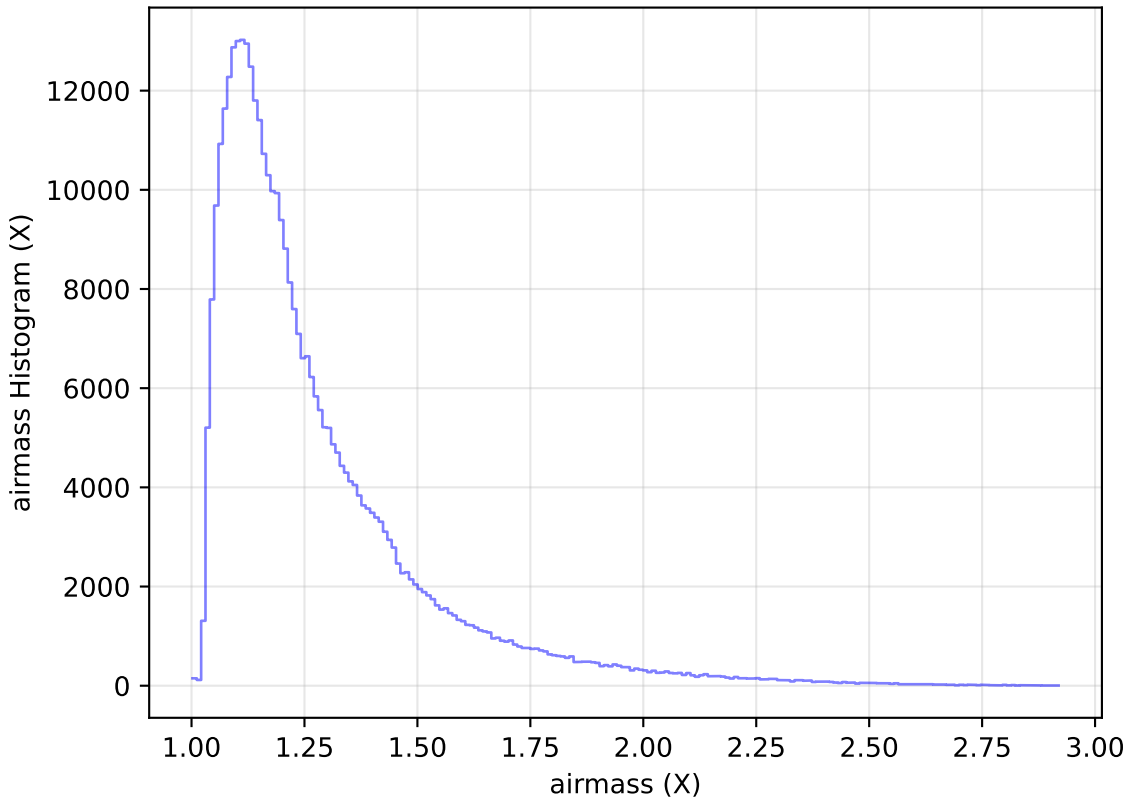
too_elab_r8_d3_gz_v3.4_10yrs WFD y band: airmass Histogram
