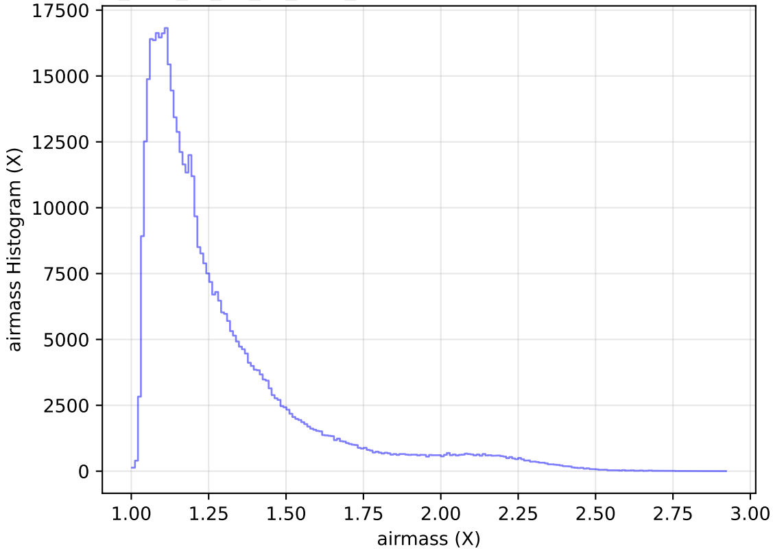
too_elab_r8_d3_gz_v3.4_10yrs WFD r band: airmass Histogram
