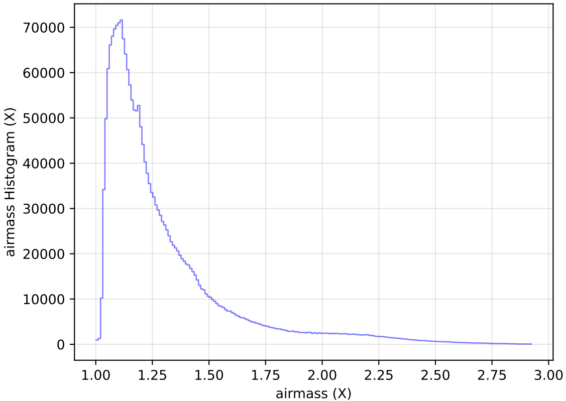
too_elab_r8_d3_gz_v3.4_10yrs WFD all bands: airmass Histogram
