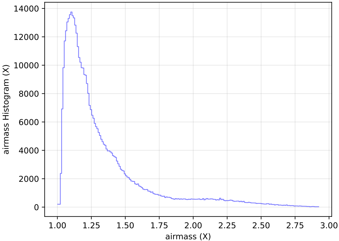
too_elab_r8_d3_gz_v3.4_10yrs All sky z band: airmass Histogram
