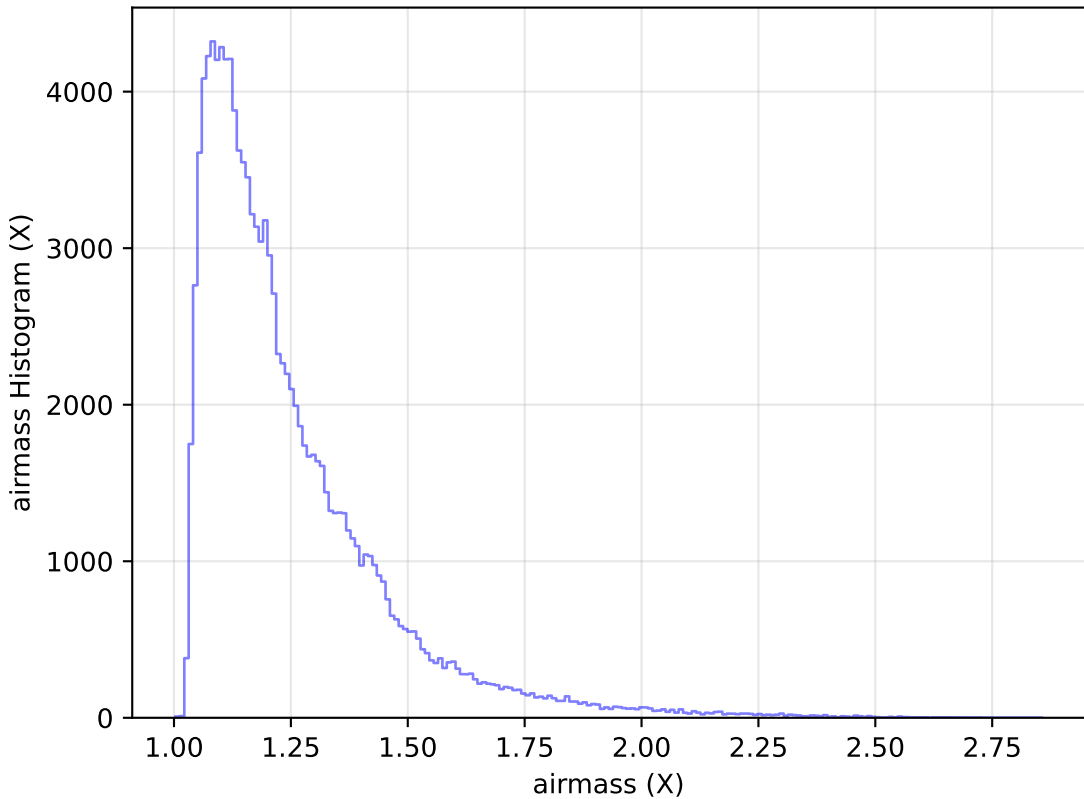
too_elab_r8_d3_gz_v3.4_10yrs All sky u band: airmass Histogram
