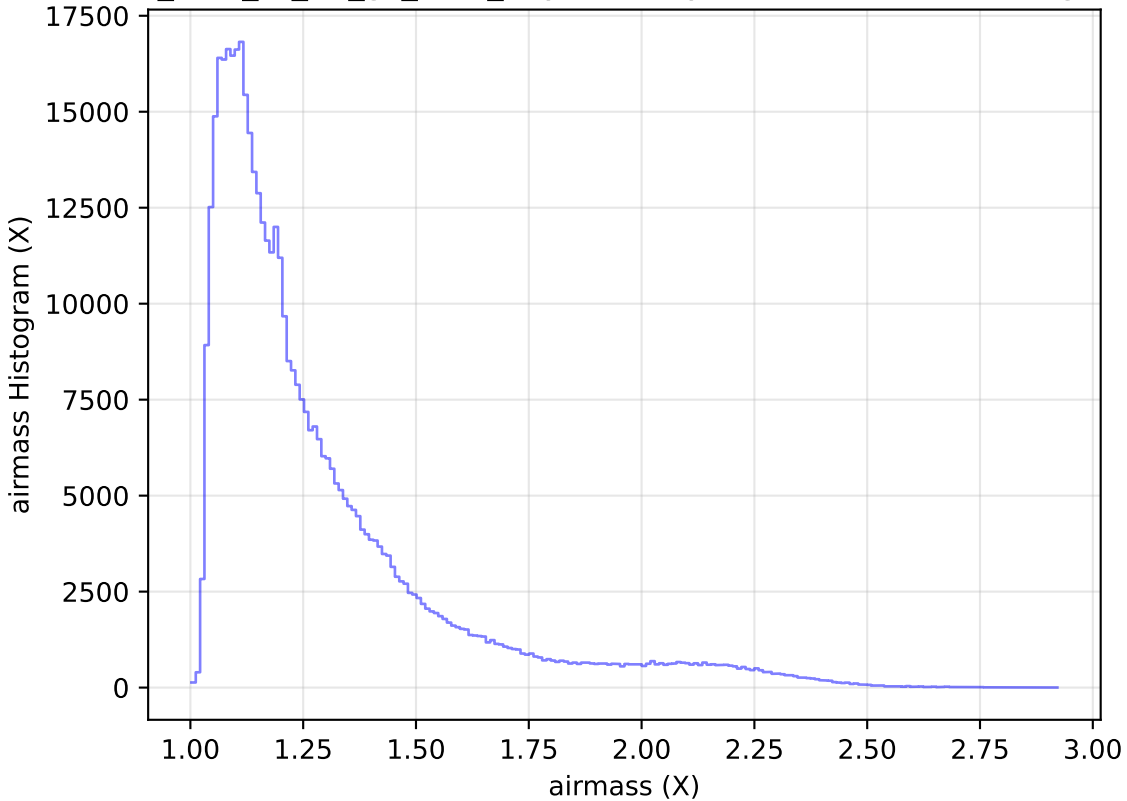
too_elab_r8_d3_gz_v3.4_10yrs All sky r band: airmass Histogram
