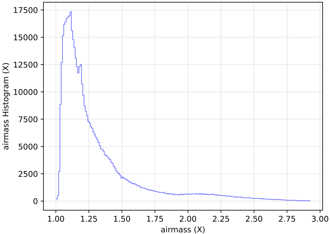
too_elab_r8_d3_gz_v3.4_10yrs All sky i band: airmass Histogram
