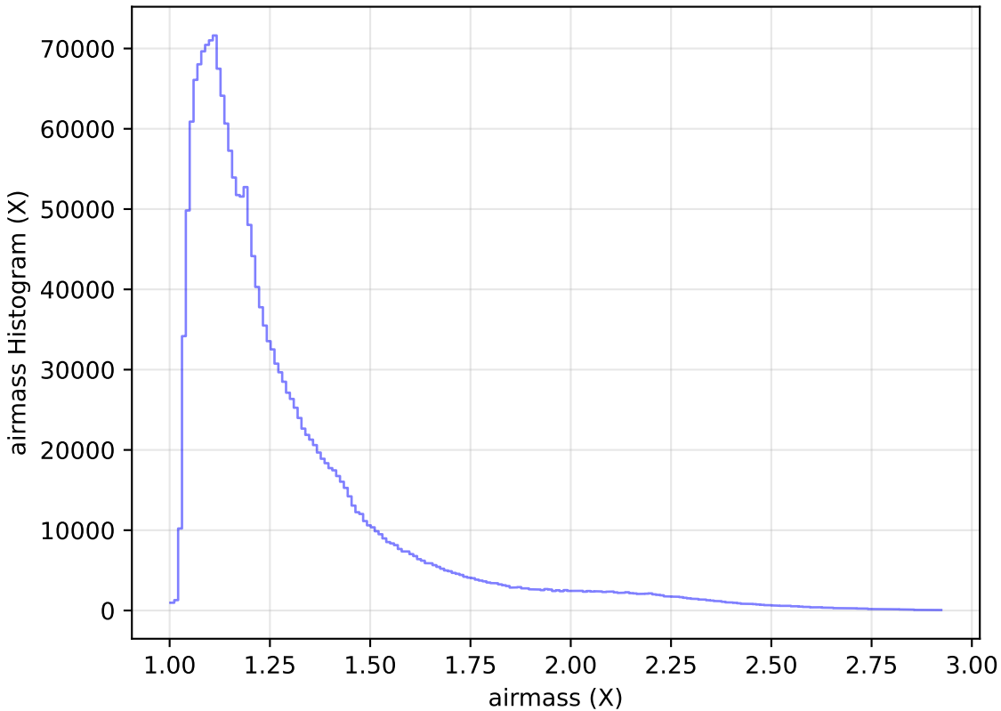
too_elab_r8_d3_gz_v3.4_10yrs All sky all bands: airmass Histogram
