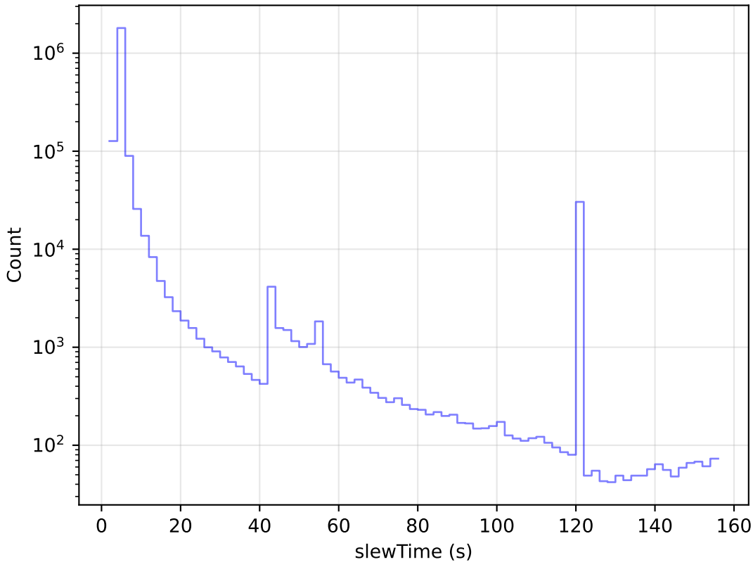
too_elab_r8_d3_gz_v3.4_10yrs All visits: Slew Time Histogram
