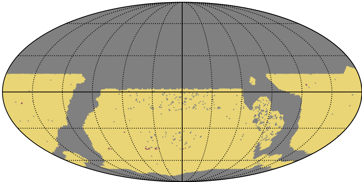
too_elab_r8_d3_gz_v3.4_10yrs WFD: RapidRevisits
