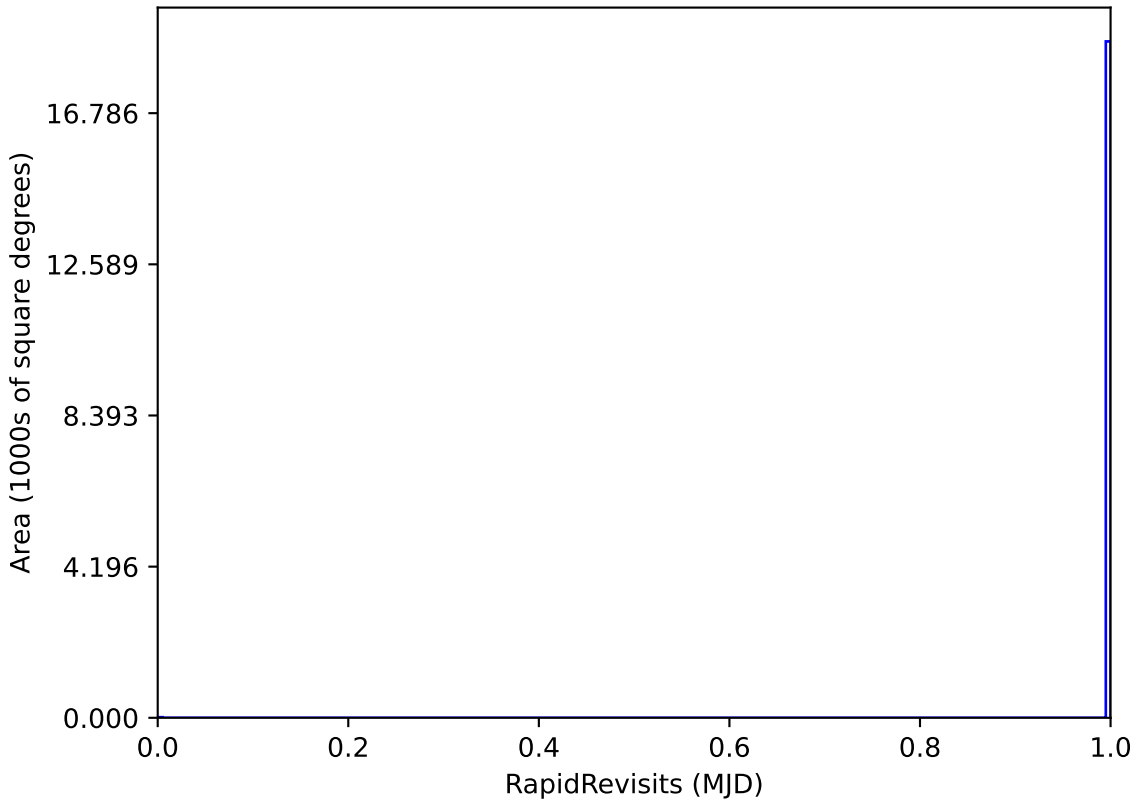
too_elab_r8_d3_gz_v3.4_10yrs WFD: RapidRevisits
