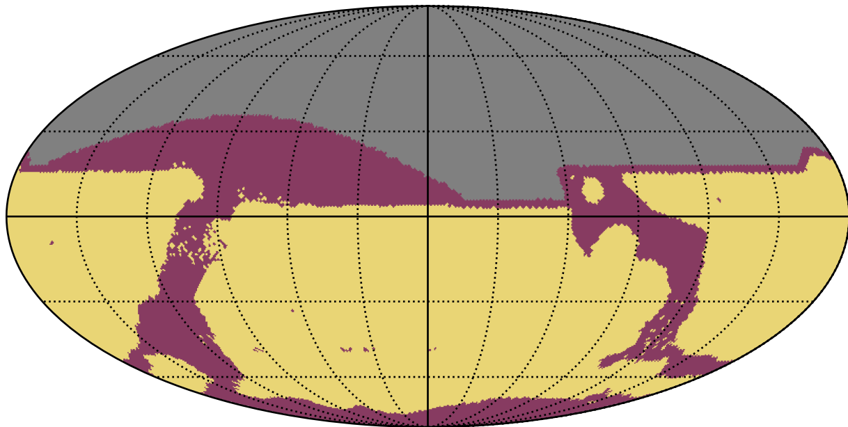
too_elab_r8_d3_gz_v3.4_10yrs All sky: RapidRevisits
