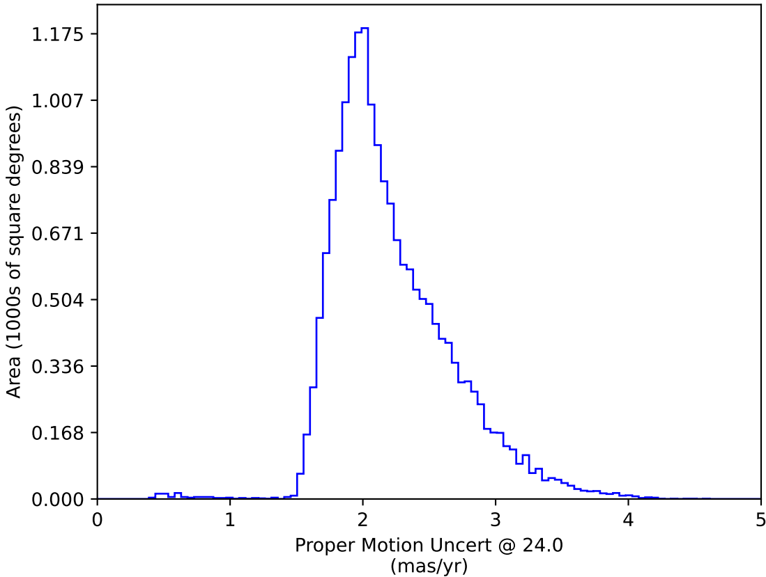
too_elab_r8_d3_gz_v3.4_10yrs WFD: Proper Motion Uncert @ 24.0
