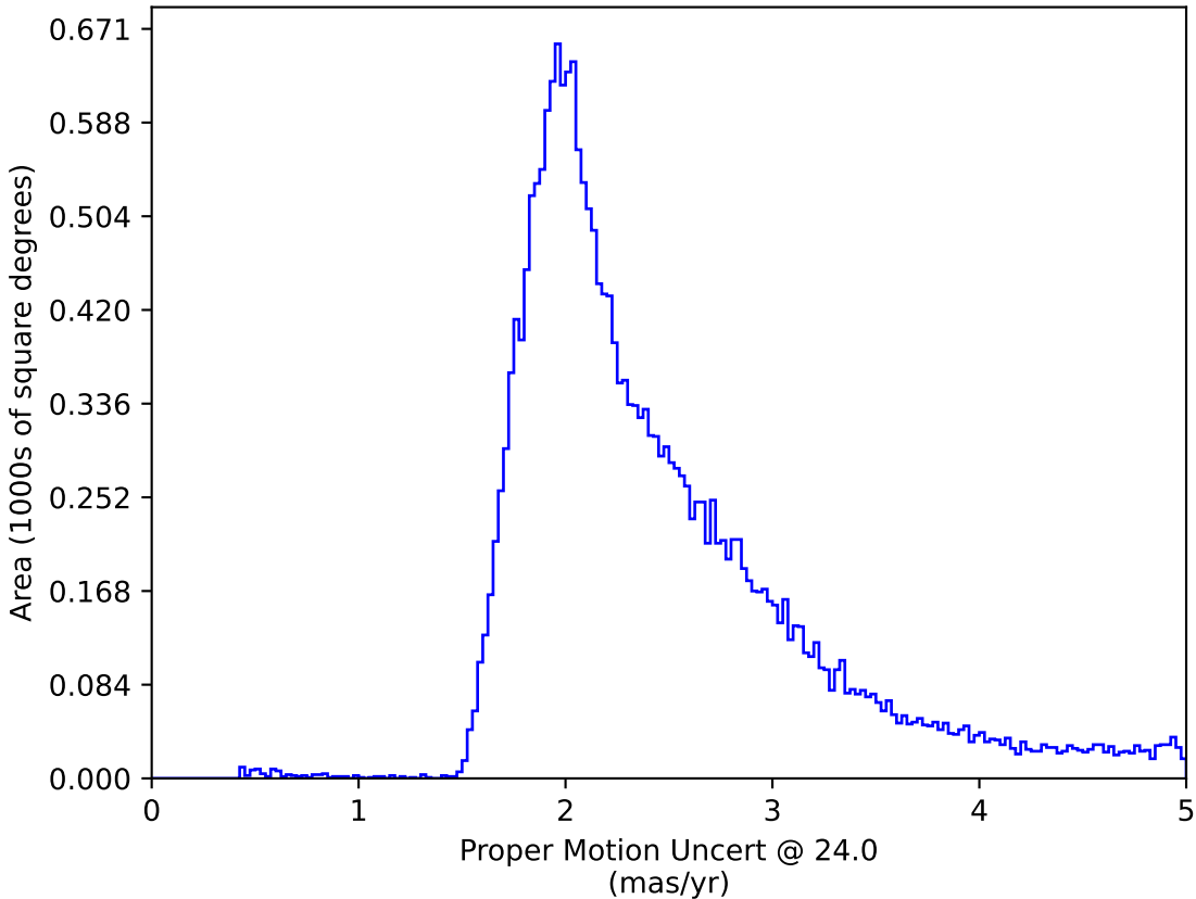
too_elab_r8_d3_gz_v3.4_10yrs All sky: Proper Motion Uncert @ 24.0
