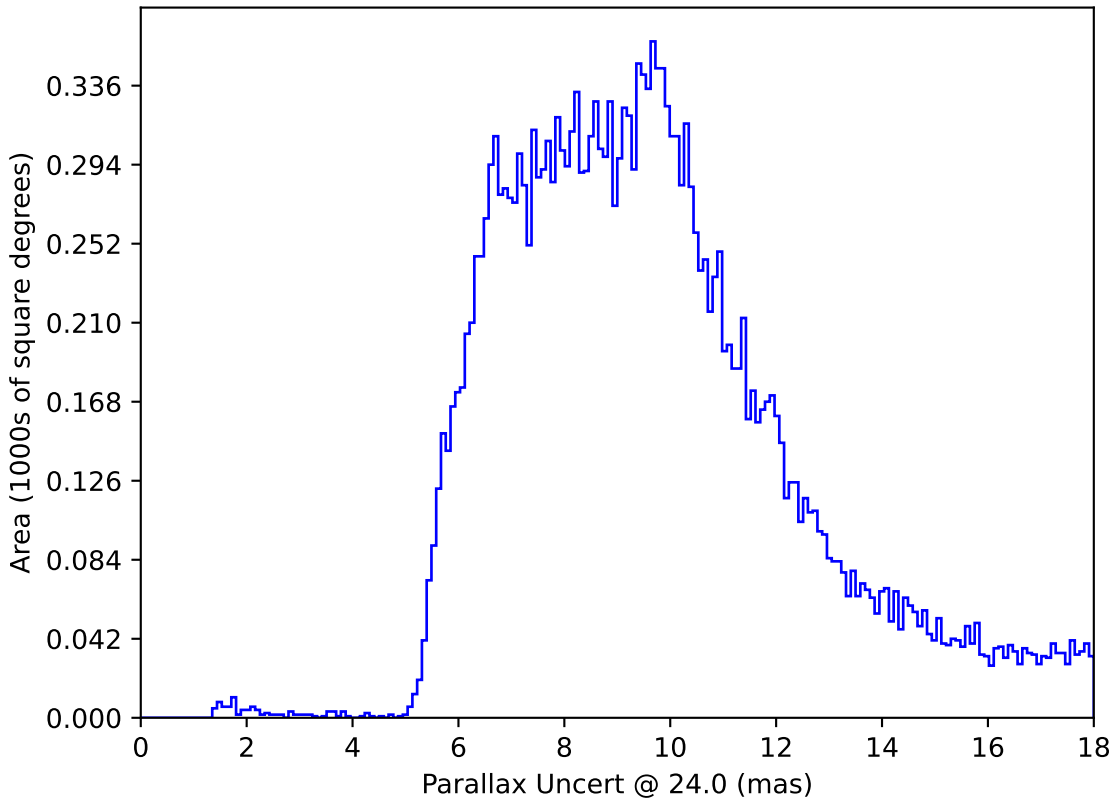
too_elab_r8_d3_gz_v3.4_10yrs All sky: Parallax Uncert @ 24.0
