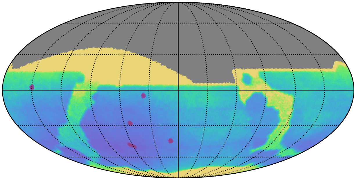
too_elab_r8_d3_gz_v3.4_10yrs All sky: Parallax Uncert @ 22.4
