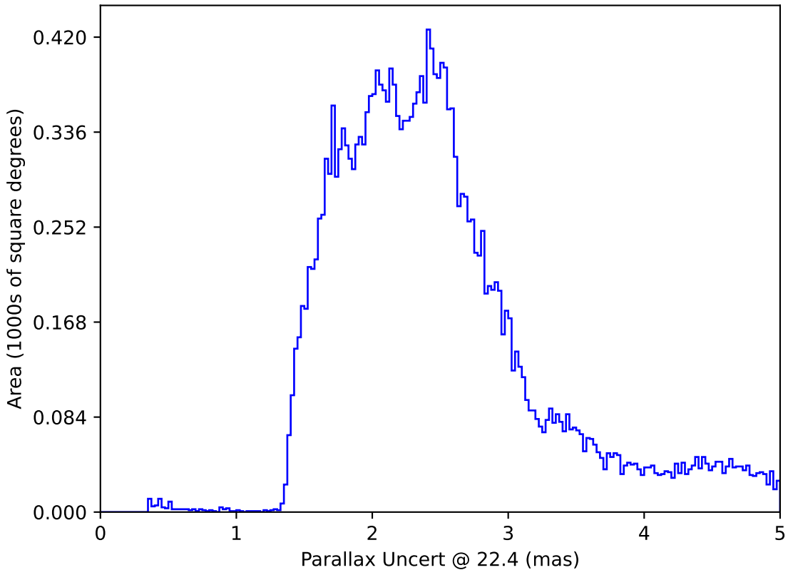
too_elab_r8_d3_gz_v3.4_10yrs All sky: Parallax Uncert @ 22.4
