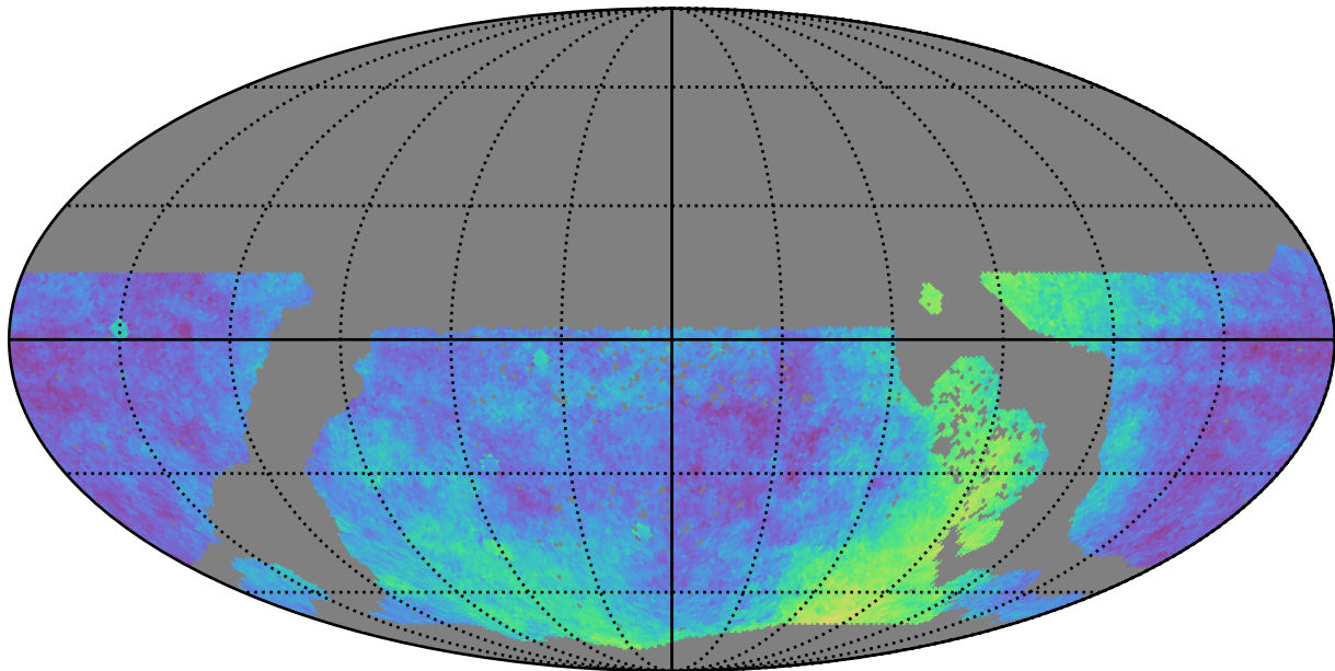
too_elab_r8_d3_gz_v3.4_10yrs WFD: Parallax Coverage @ 24.0
