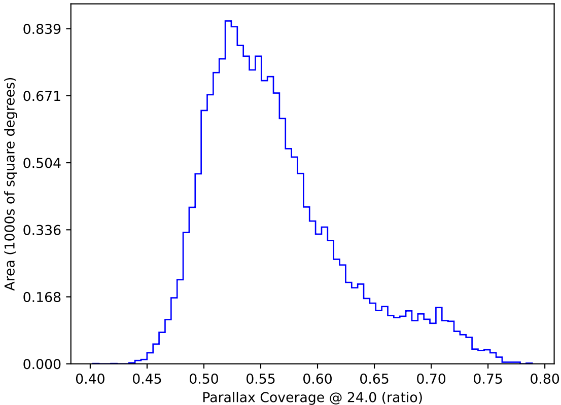
too_elab_r8_d3_gz_v3.4_10yrs WFD: Parallax Coverage @ 24.0
