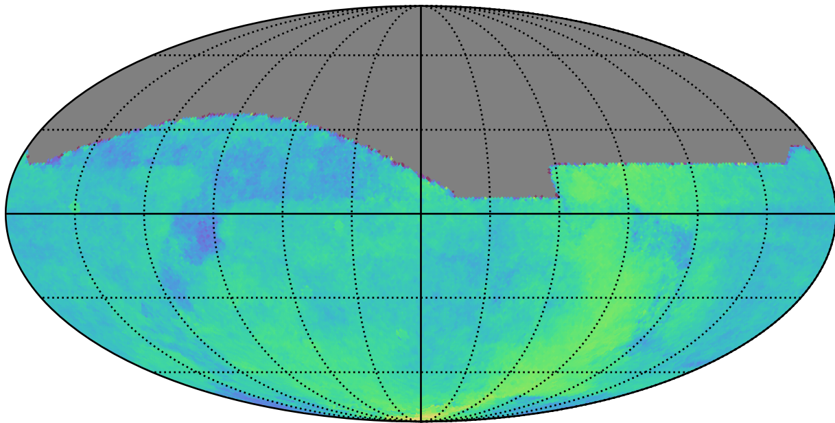
too_elab_r8_d3_gz_v3.4_10yrs All sky: Parallax Coverage @ 24.0
