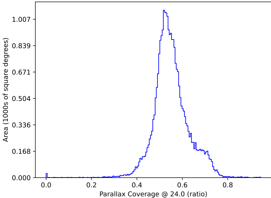
too_elab_r8_d3_gz_v3.4_10yrs All sky: Parallax Coverage @ 24.0
